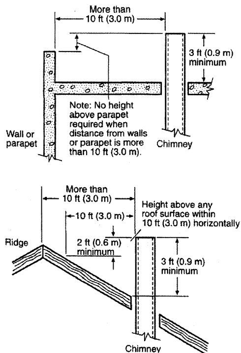
FIGURE 5-1 Typical Termination Locations for Chimneys and Single-Wall Metal Pipes Serving Residential-Type and Low-Heat Appliance [NFPA 54: Figure 12.6.2.1]
